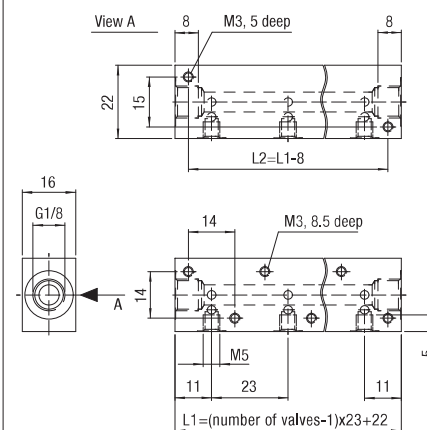
Collector plate
